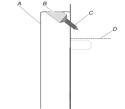
A. Trim kit frame B. Mounting hole guide C. #7-16x15/16" flat head wood screw (4) D. Cutout ceiling
