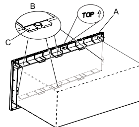
A. Trim Kit Frame B. Locating pin (4) C. Locating slot (4)
